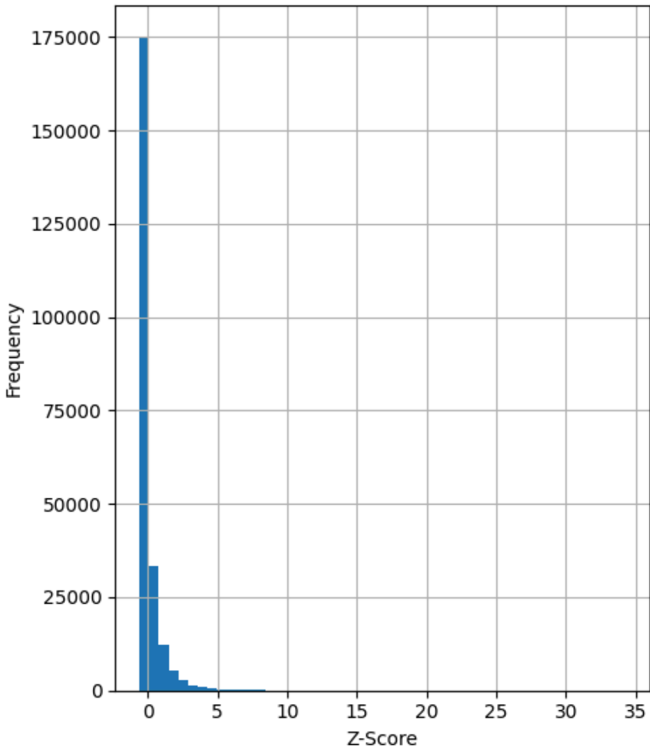
Z-Score Distribution
